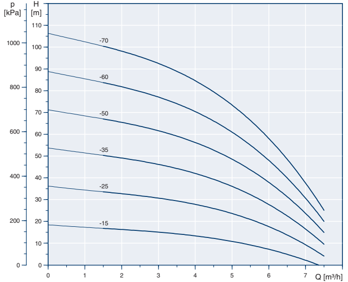
SQ/SQE 5 ISO 9906 Annex A
