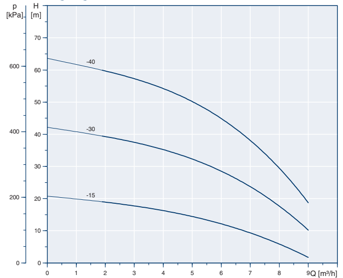
SQ/SQE 7 ISO 9906 Annex A
