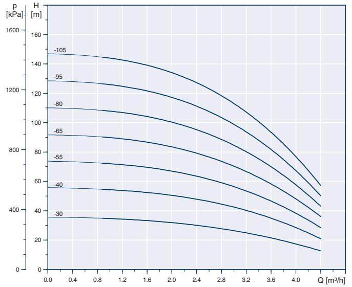
SQ/SQE 3 ISO 9906 Annex A
